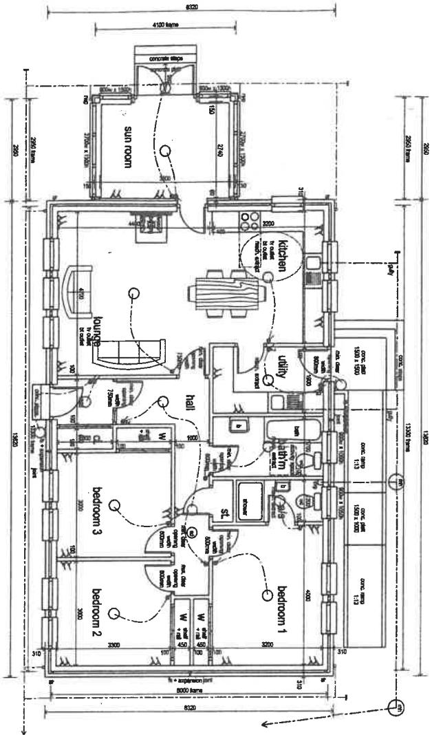
floor plan.
